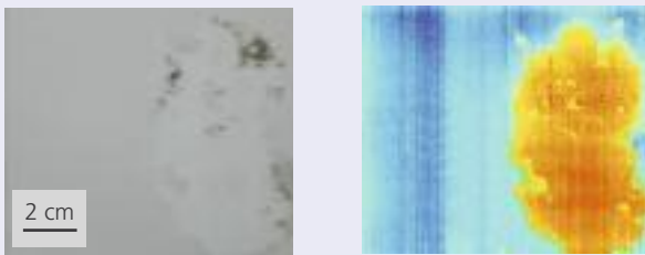
Visualization and clear chemical statistical identification (right) of a grease contaminated steel substrate (left)
