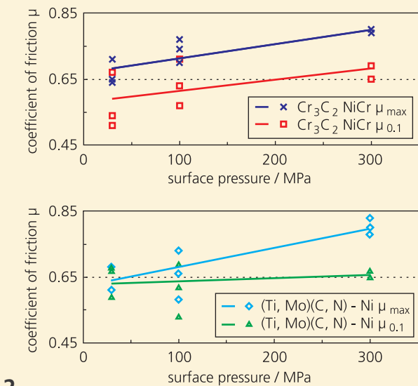
Dependence of the friction coefficients \mu_{0,1} and \mu_{max} as a function of the contact pressure for \text{Cr}_3\text{C}_2\text{-NiCr} and (\text{Ti}, \text{Mo})(\text{C}, \text{N})\text{-Ni} coatings
