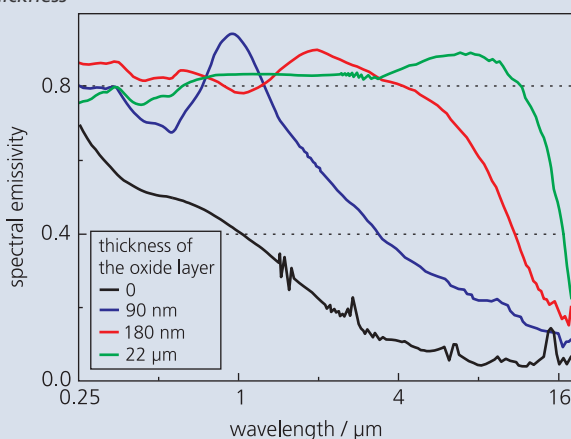
Spectral emissivity of steel 42CrMo4 as a function of oxide film thickness
