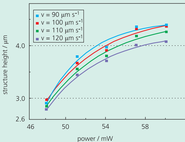
Structure height as a function of process speed and laser power during 2-photon polymerization of OrmoComp®
