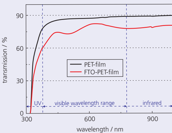
Transmission of a FTO-PET foil compared to an uncoated foil.
