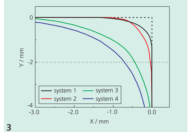
X-Y-plot during generation of a 90° corner with target speed of v = 15 \text{ m s}^{-1}
