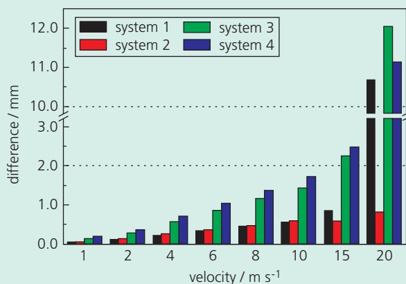
Contour deviation when generating a 90° corner with different scanner systems
