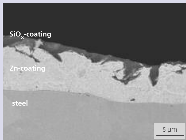
Scanning electron microscopic cross section of the coating design of dip-galvanized steels after vacuum suction blasting
