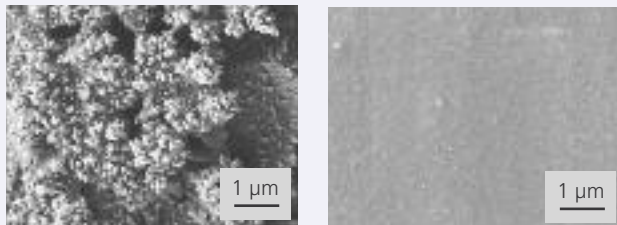
SEM image of nanostructured \text{SiO}_2 coatings on TiAl6V4 for structural bonding (left) and as a barrier coating (right)
