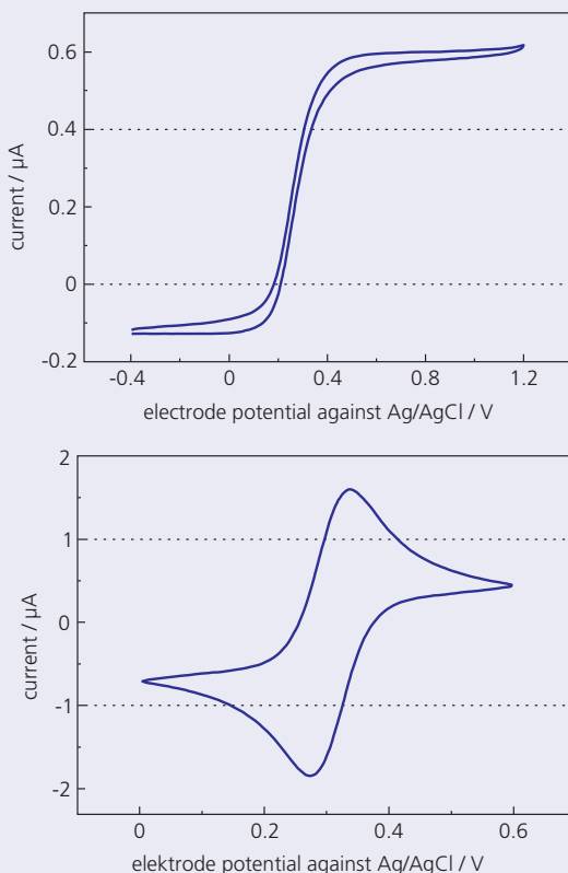
Cyclic voltammograms of a MEA (1 mM K_4Fe(CN)_6 in 0.1 M KCl, top) and of a macro electrode (1 mM K_4Fe(CN)_6 in 1 M KCl, bottom)
