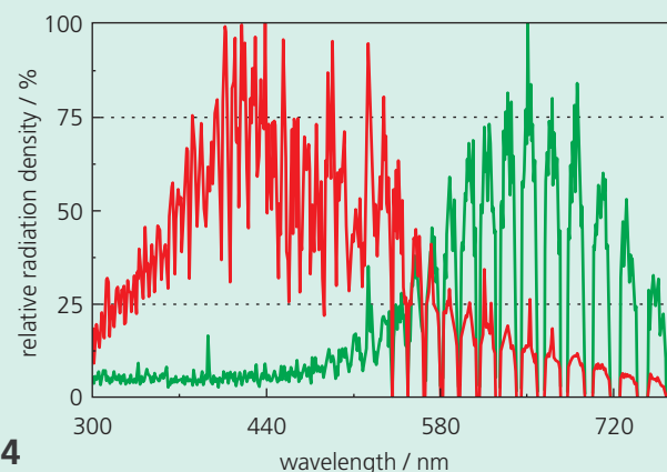
Spectra of unstable (red) and stable (green) cutting processes using a 4 kW fiber laser (steel substrate X5CrNi18-10, thickness 12 mm)
