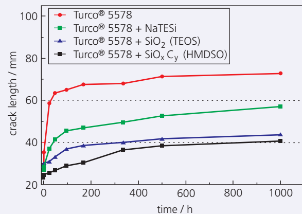
Result of the wedge test according to DIN 65448, the crack propagation is plotted versus time on pretreated TiAl6V4
