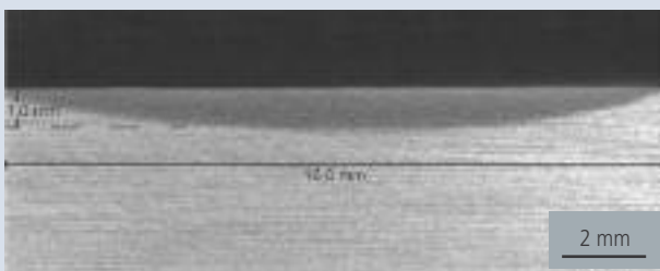
Cross section of a hardened 42CrMo4 component (focus spot 20 x 8 mm 2 ) and hardness-depth curve
