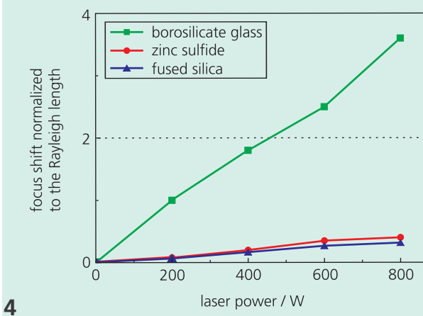
Laser induced focus shift of imaging optics different substrate materials
