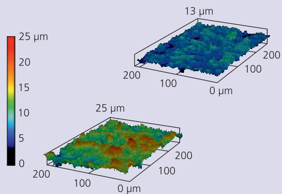
Topographies of treated surfaces top – SACO®-vacuum suction blasting bottom – SACO®-pressure blasting
