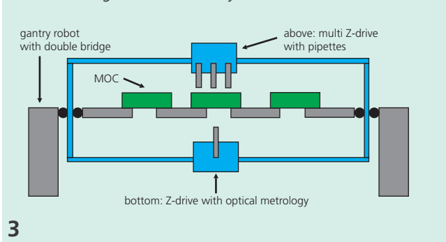
Schematic design of the laboratory automation
