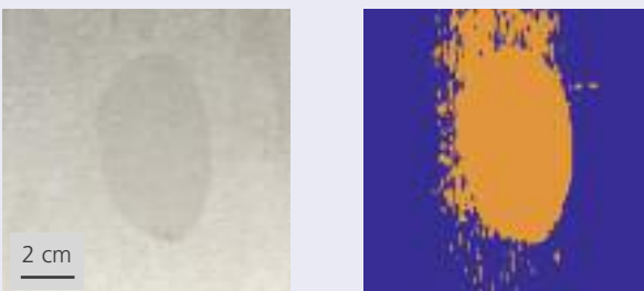
Visualization and clear chemical statistical identification (right) of a grease contaminated steel substrate (left)
