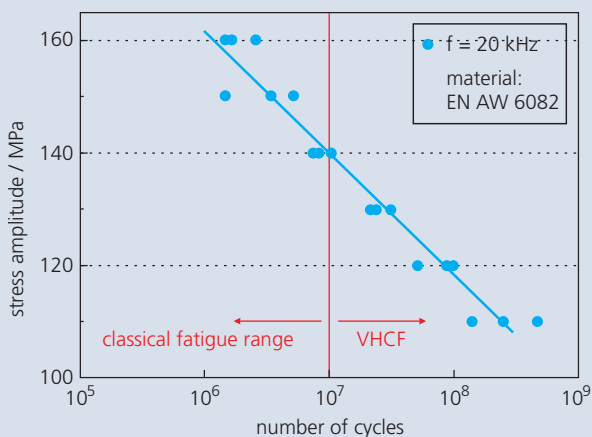
S-N-curve showing the fatigue strength up to crack initiation measured by means of an ultrasonic fatigue test system at a stress ratio of R = 1
