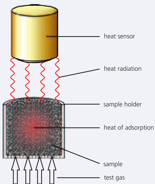
Measurement principle for the quick test method
